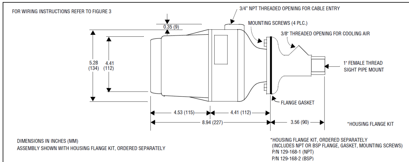
FIGURE 2. SIMPLICITY SCANNER in CENELEC HAZARDOUS AREA HOUSING (mounting flange kit ordered separately)
