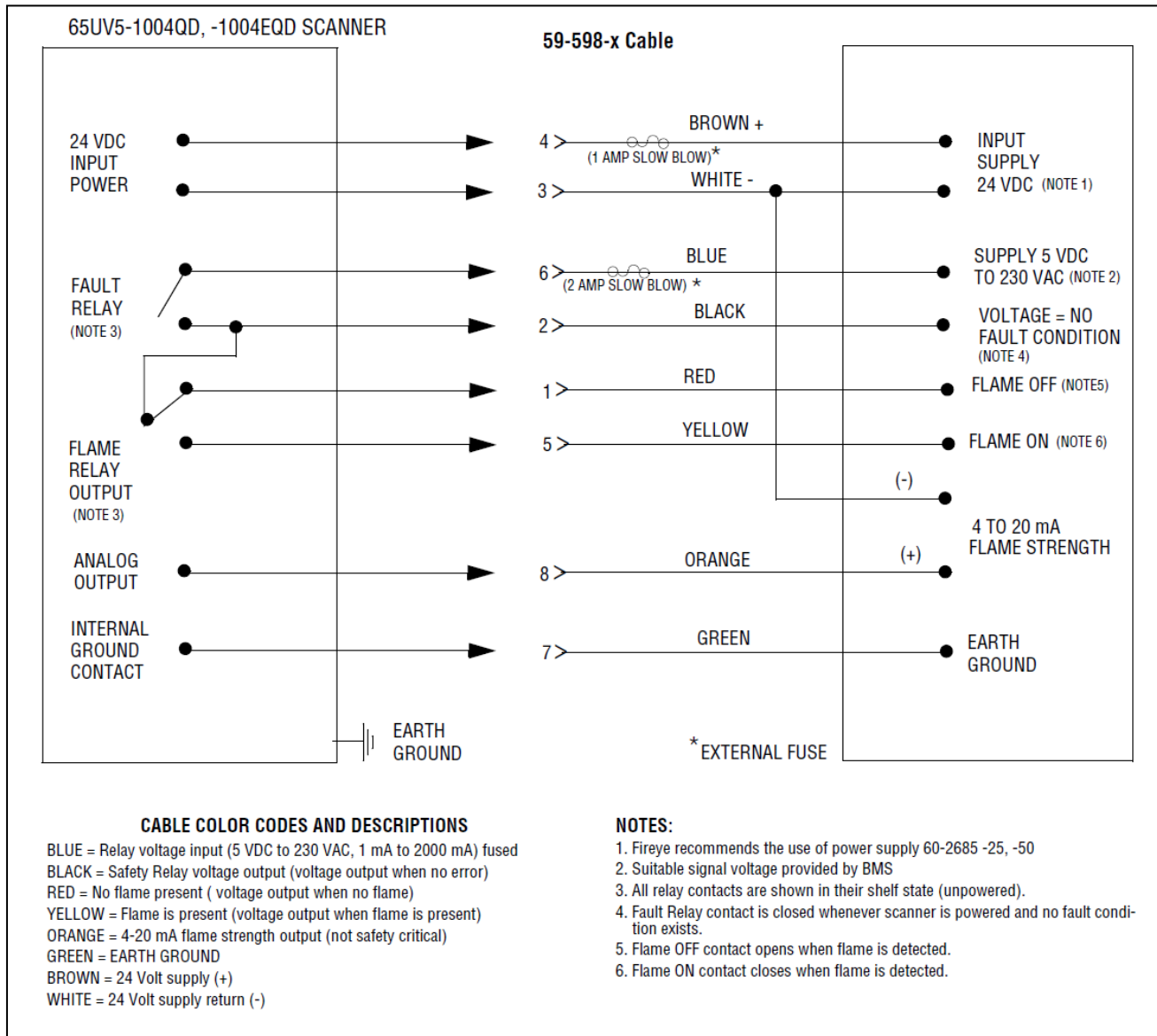
FIGURE 9. SCANNER WIRING FOR 1004QD AND 1004EQD SCANNER VERSIONS
