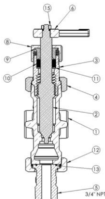
LOWER VALVE
