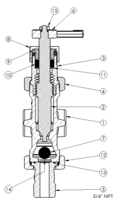
UPPER VALVE
