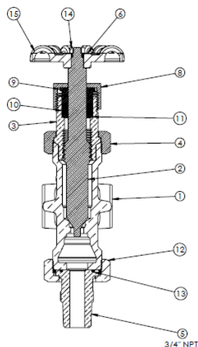
LOWER VALVE
