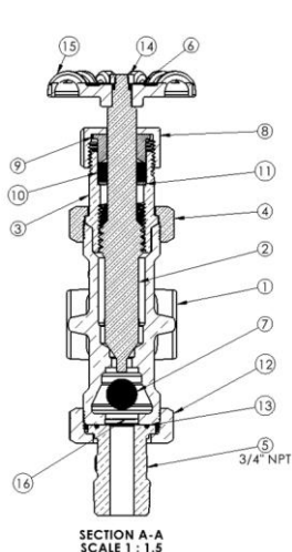
UPPER VALVE
