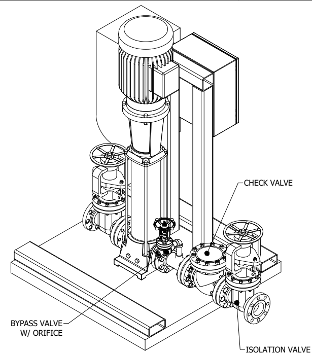
ISO FRONT LEFT (DISCHARGE SIDE)
